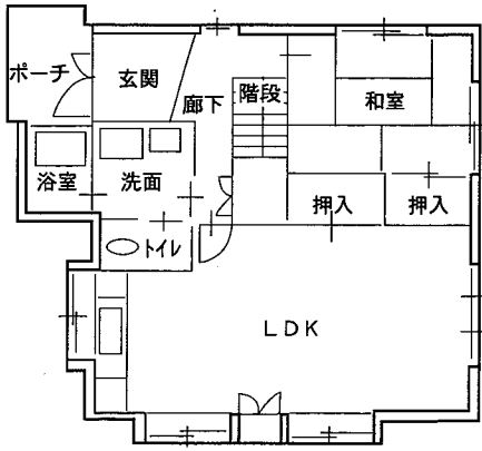
1F
